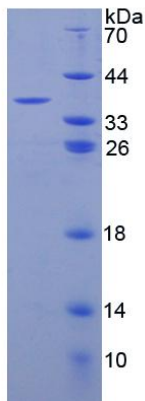
Figure 2. SDS-PAGE
